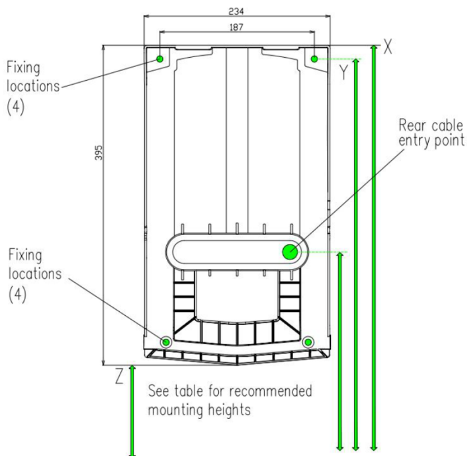
REAR ELEVATION
